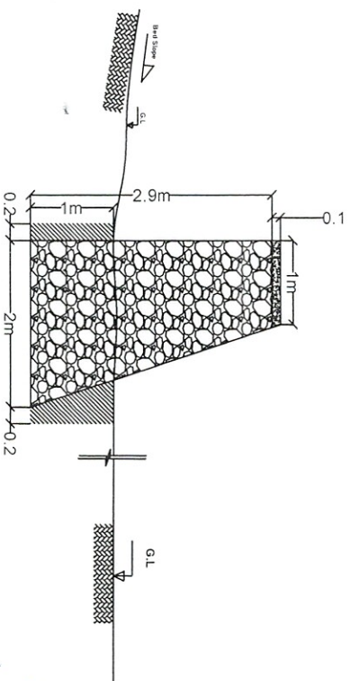
Section B3-B3 Scale 1:50
